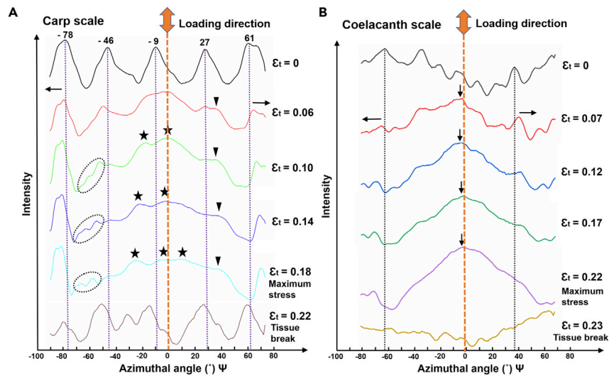
Figure 8. Quantification of the Rotation of Collagenous Lamellae for the Carp Scale under Tensile Loading in Comparison with That for the Coelacanth Scale
